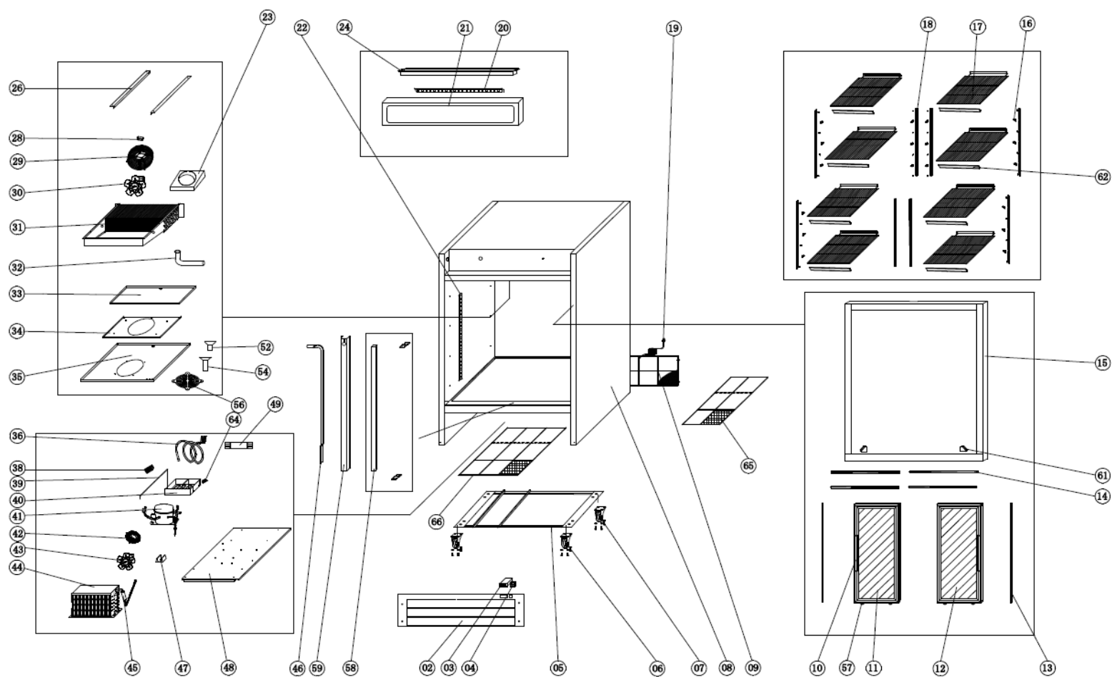
EXPLODED VIEW OF KCHSGM48R
